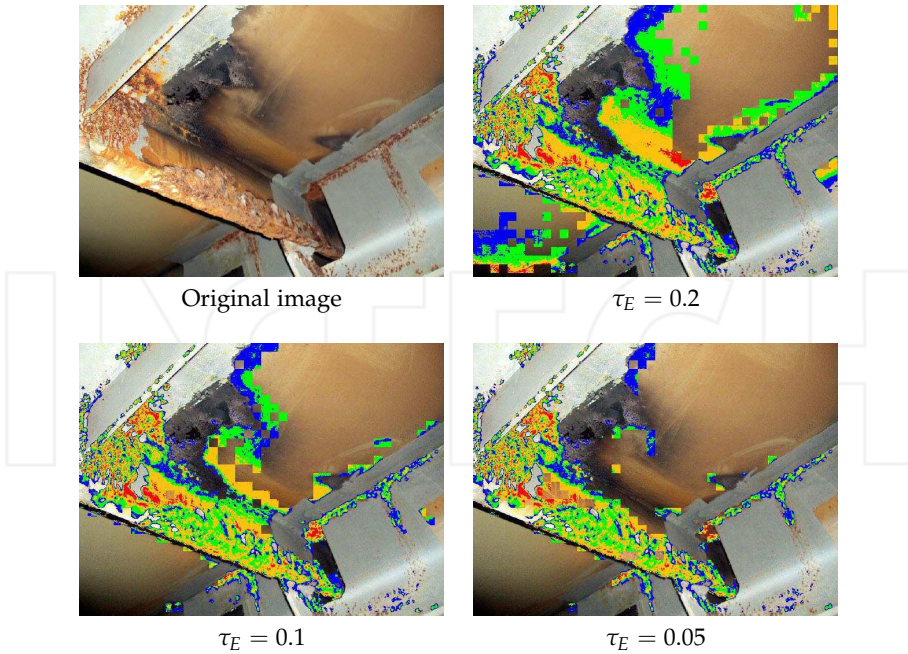
Figure 2. Corroded areas detected by WCCD for different energy threshold values
